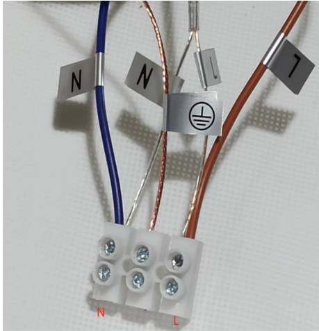
Step 5: Corresponding wire connection.
